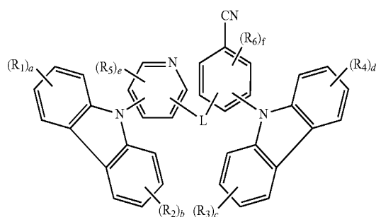
Formula 1-3
