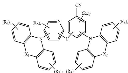
Formula 1
