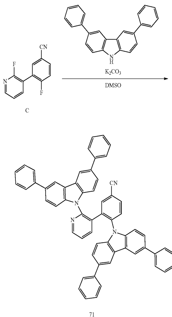
Reaction 3
