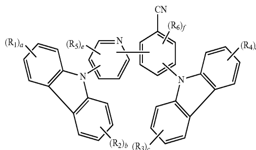
Formula 1-2
