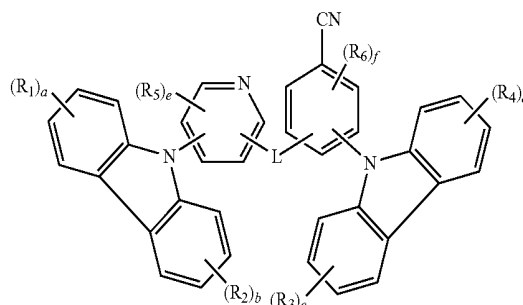
Formula 1-3
