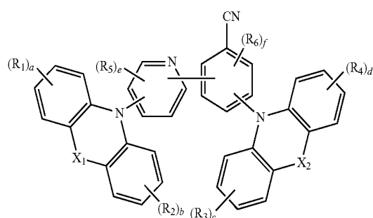
Formula 1-3
