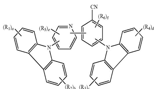
Formula 1-2
