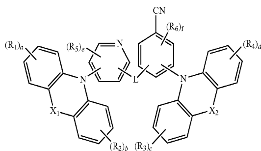
Formula 1
