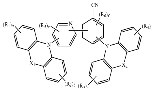
Formula 1-3
