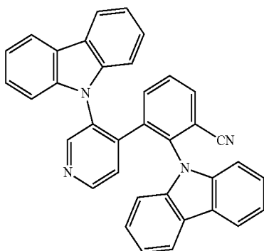
Compound Group 1
