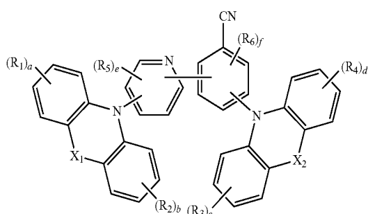
Formula 1-3
