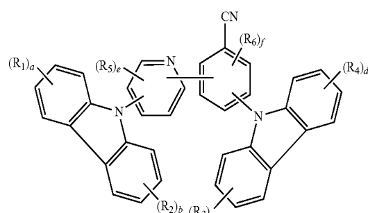
Formula 1-1
