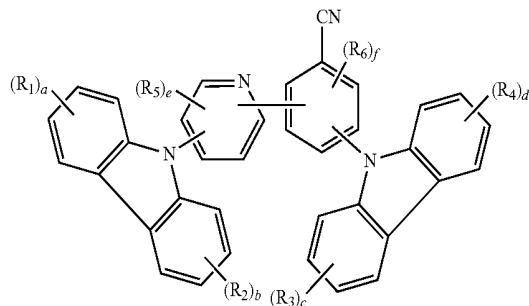
Formula 1-1
